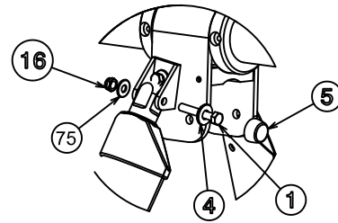
Detail D
