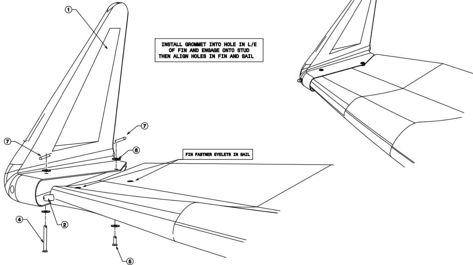
ASSEMBLED VIEW
