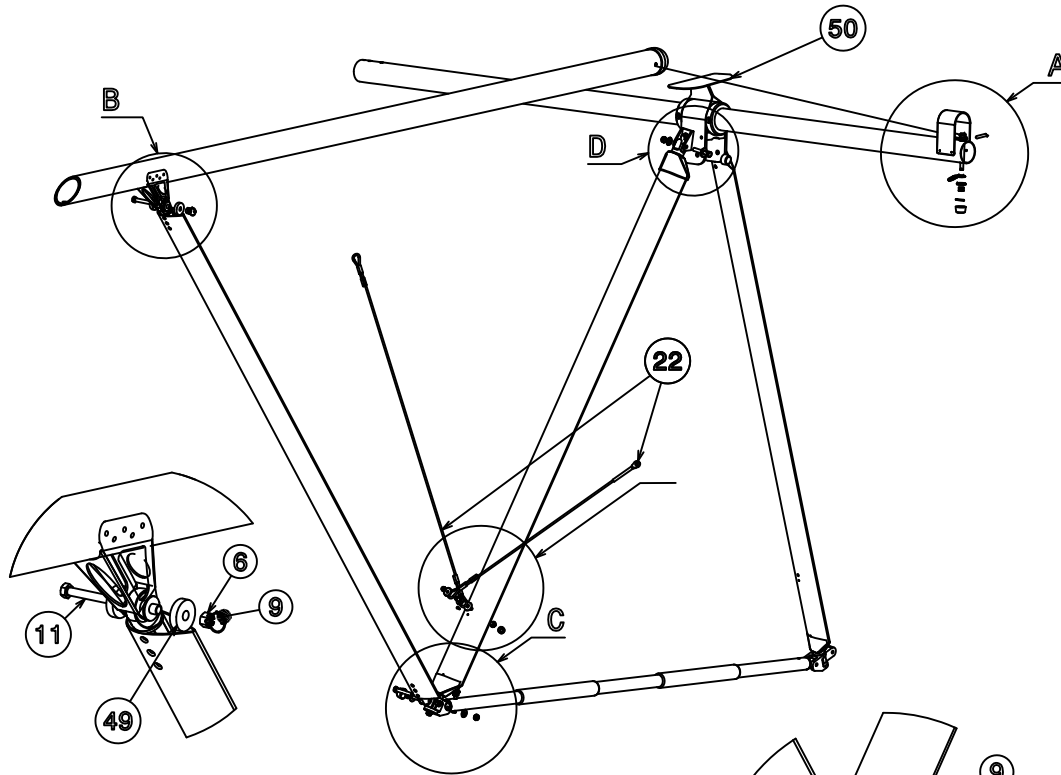
Detail B
