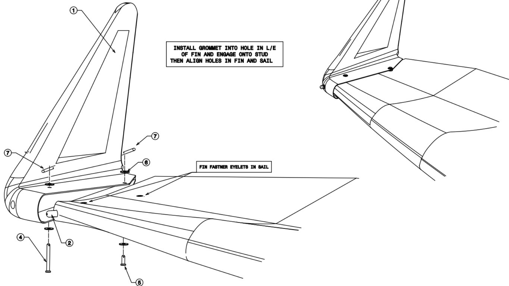
ASSEMBLED VIEW
